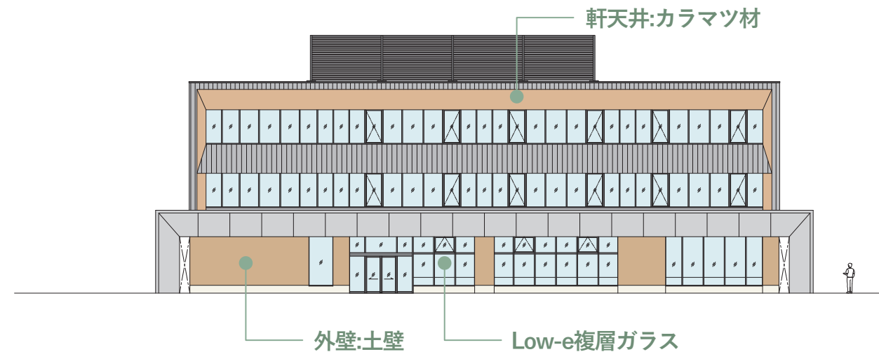
S=1/300 [南立面図]
