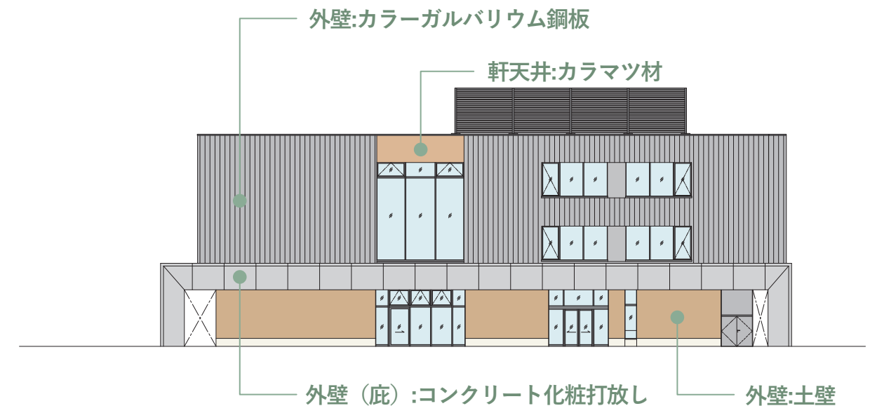
S=1/300 [東立面図]
