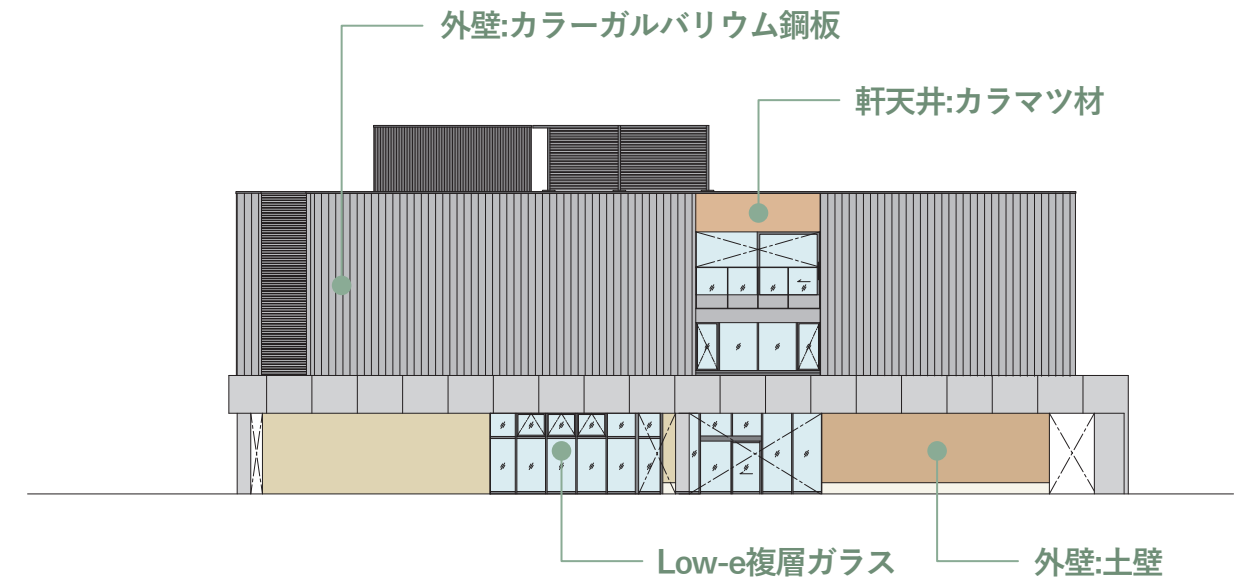
S=1/300 [西立面図]
