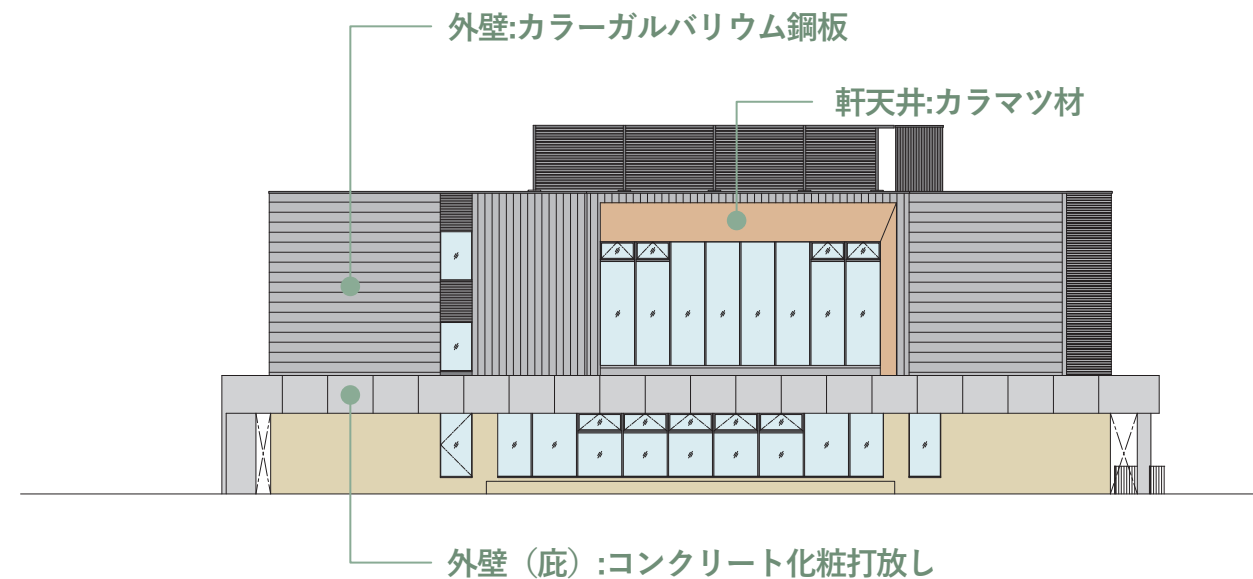
S=1/300 [北立面図]
